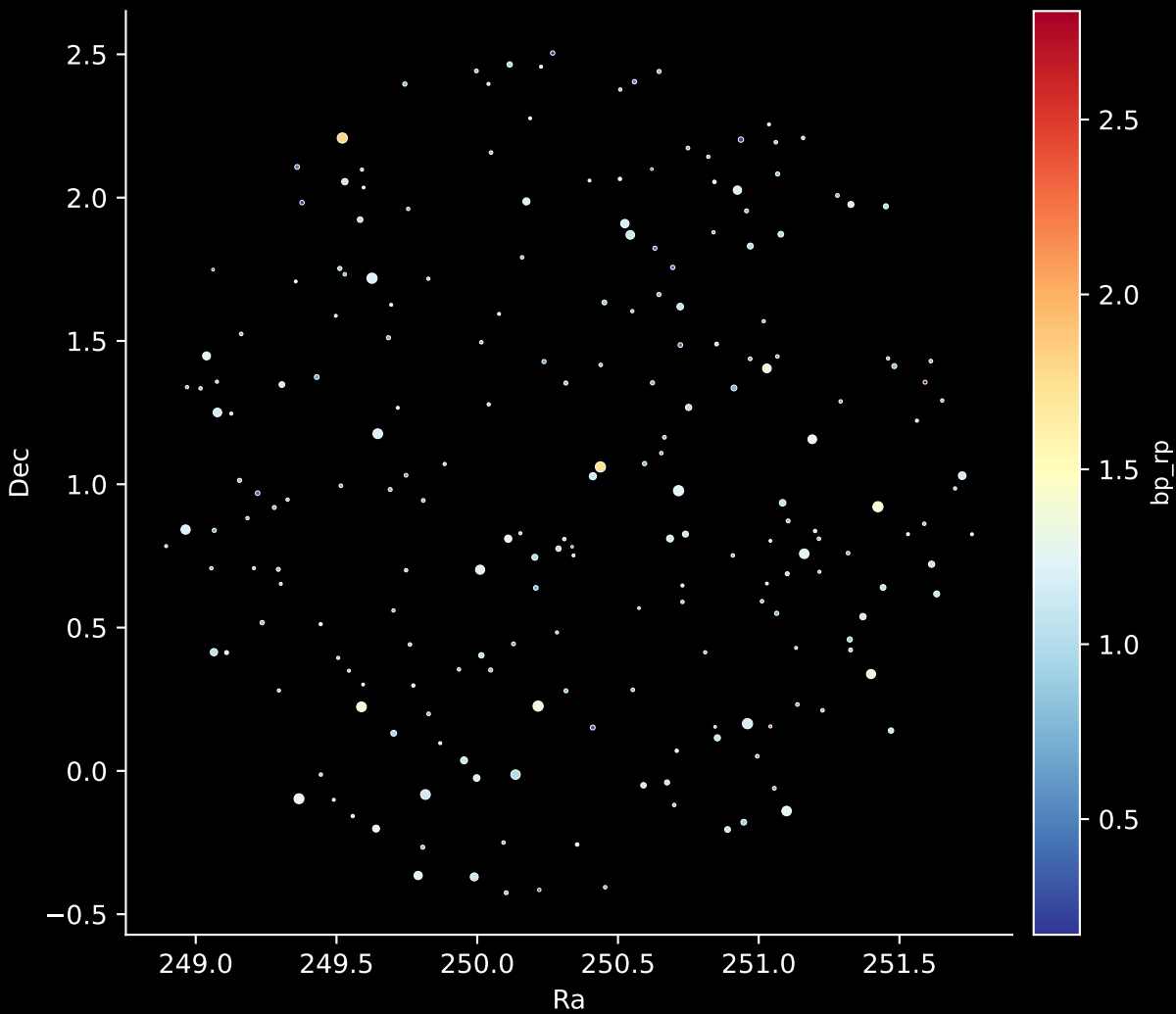
APOGEE DR17 Field: [238+42_MGA] Stars: 214
