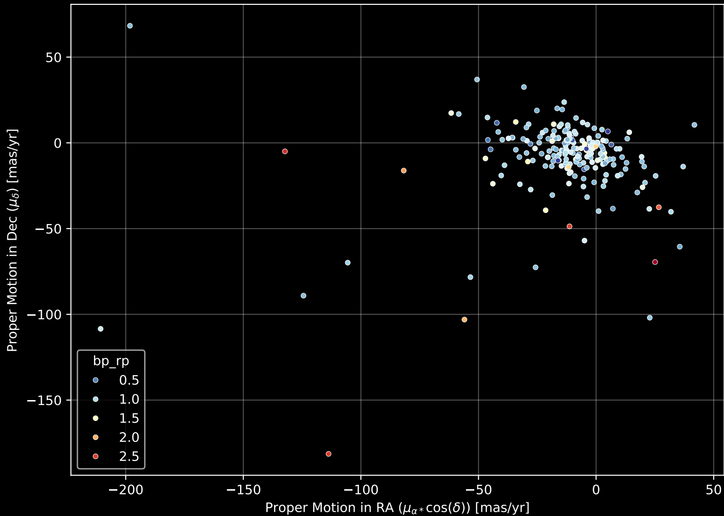
APOGEE DR17 Field: [238+42_MGA] Proper Motion Diagram (n= 214)
