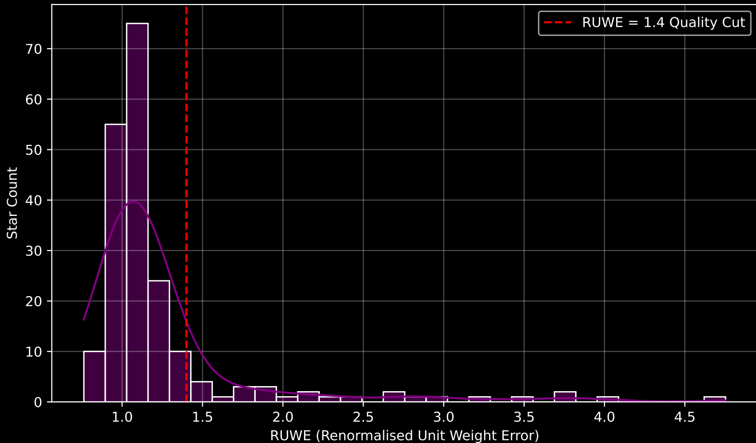
GAPOGEE DR17 Field [238+42_MGA] RUWE Distribution (n= 200)
