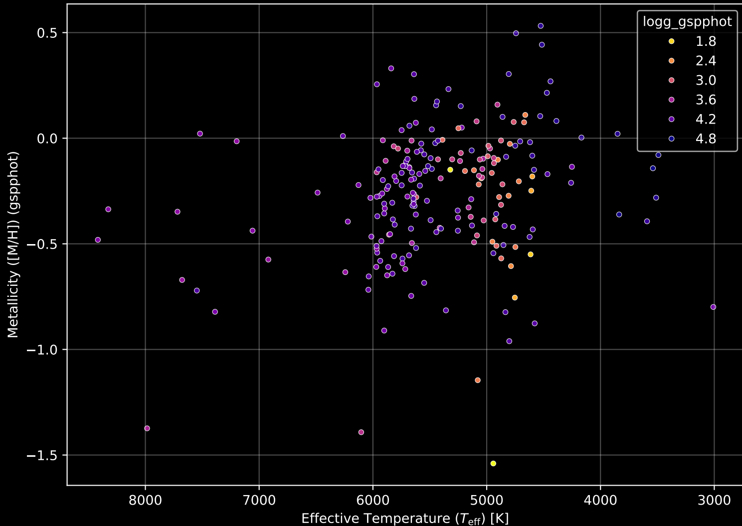
APOGEE DR17 Field: [238+42_MGA] Stellar Population Parameters (n= 214)
