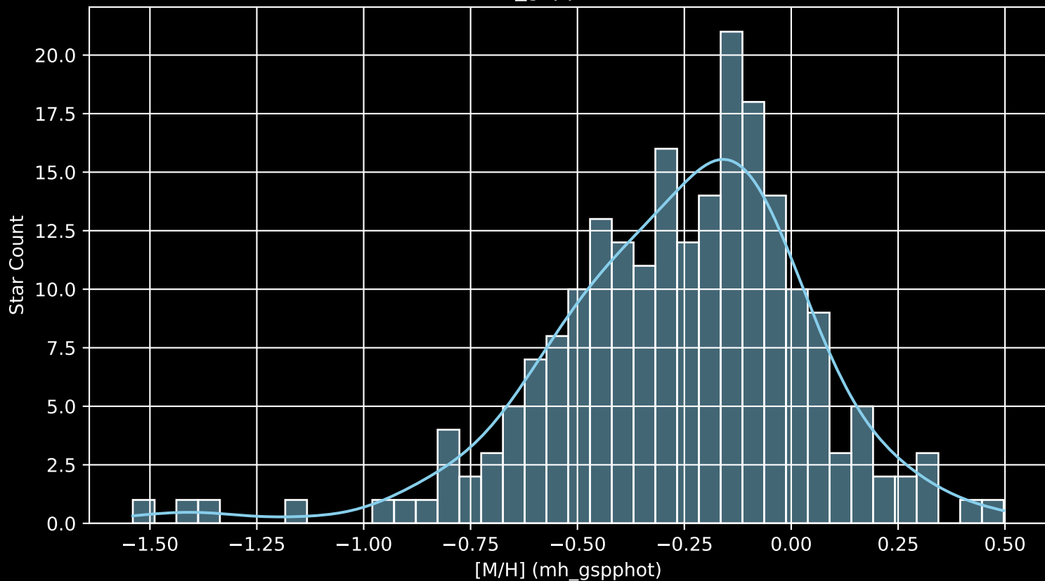
APOGEE DR17 Field: [238+42_MGA [M/H] (mh_gspphot) (n= 213)
