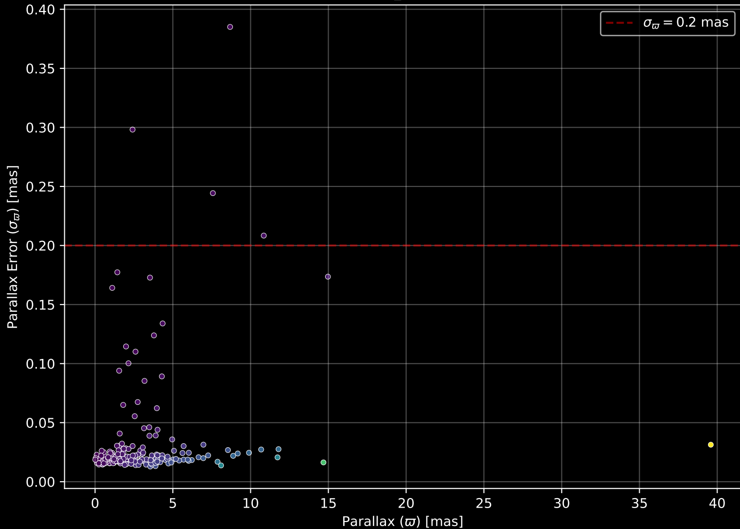
APOGEE DR17 Field: [238+42_MGA] Parallax Quality (n= 214)
