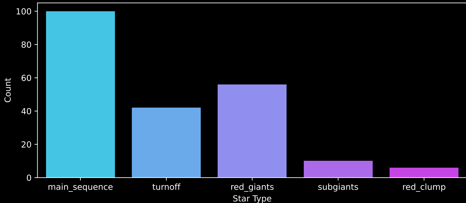
APOGEE DR17 Field: [238+42_MGA] Count plot of Star Type
