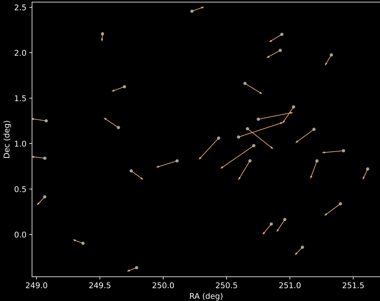
APOGEE DR17 Cluster 3 Proper Motion Vectors (n=30)
